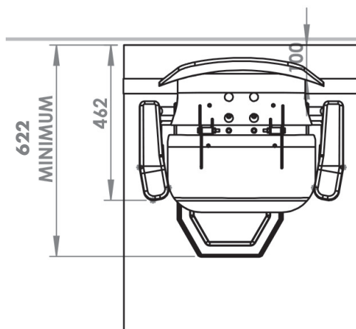
Travel Position
