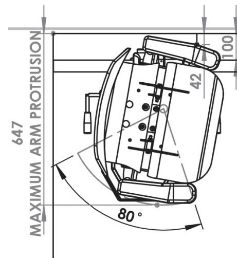
Swivel Position
